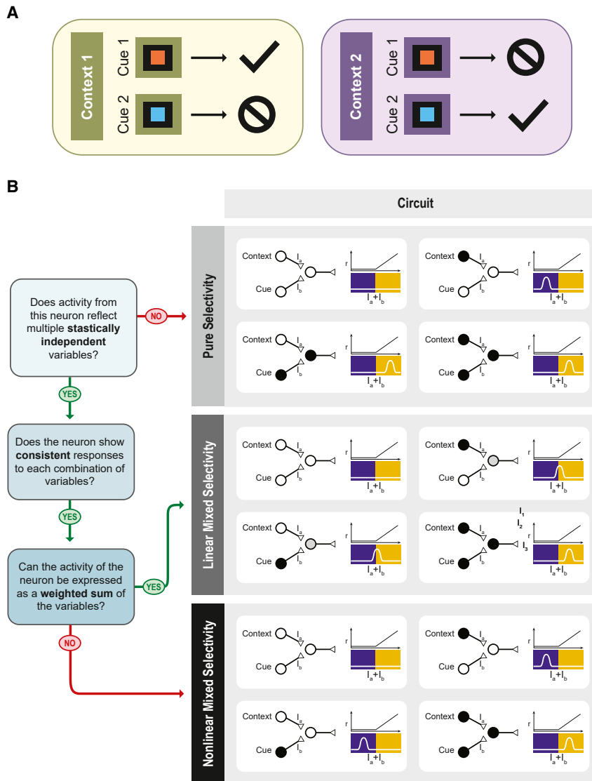
Figure 1. Delineating pure, linear mixed, and nonlinear mixed selectivity using a context-dependent task
